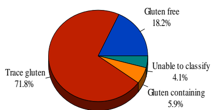
Figure 1: Proportion of subjects on each diet
